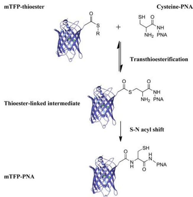
Scheme 1. mTFP-PNA Ligation Using Native Chemical Ligation (NCL) a
